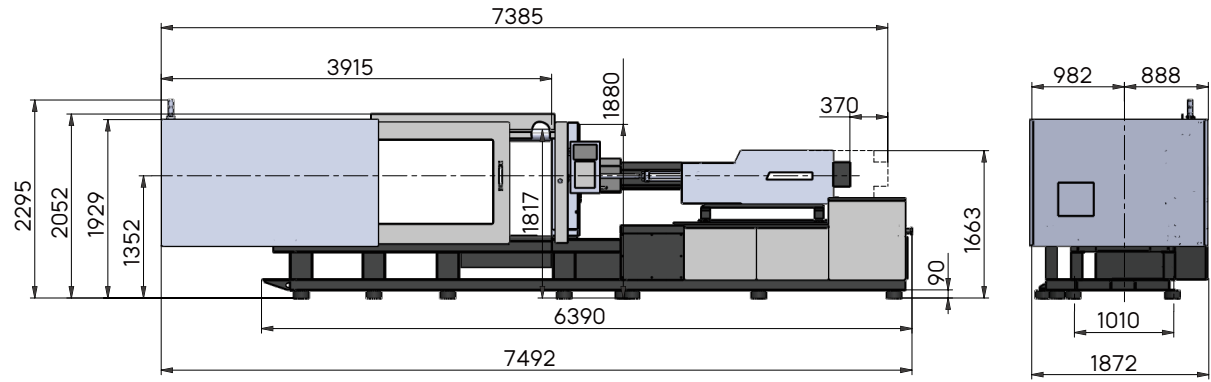
UN380SKIII
