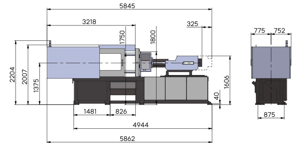
UN260SKIII
