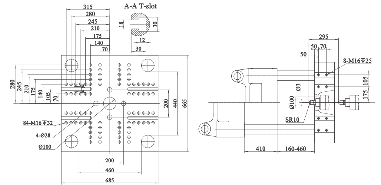
UN160SKIII
