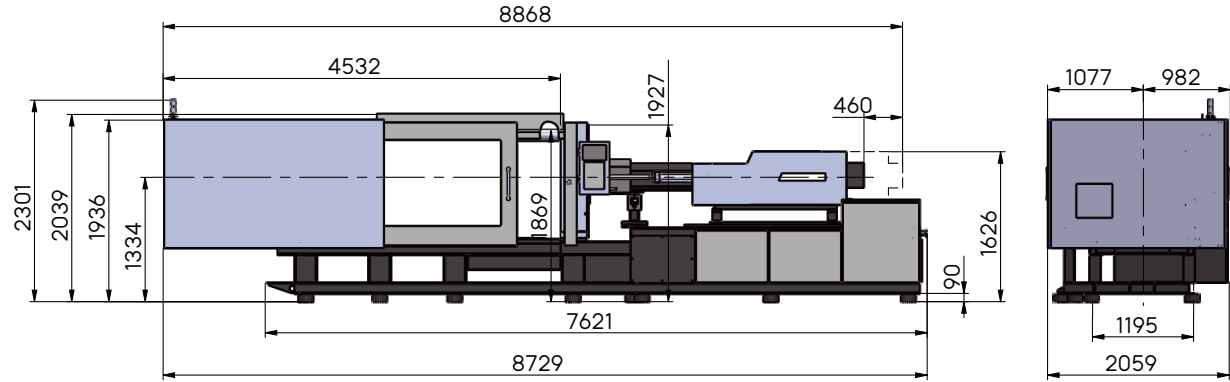
UN530SKIII
