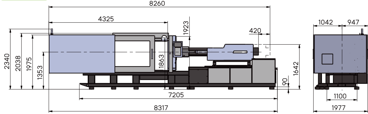
UN450SKIII
