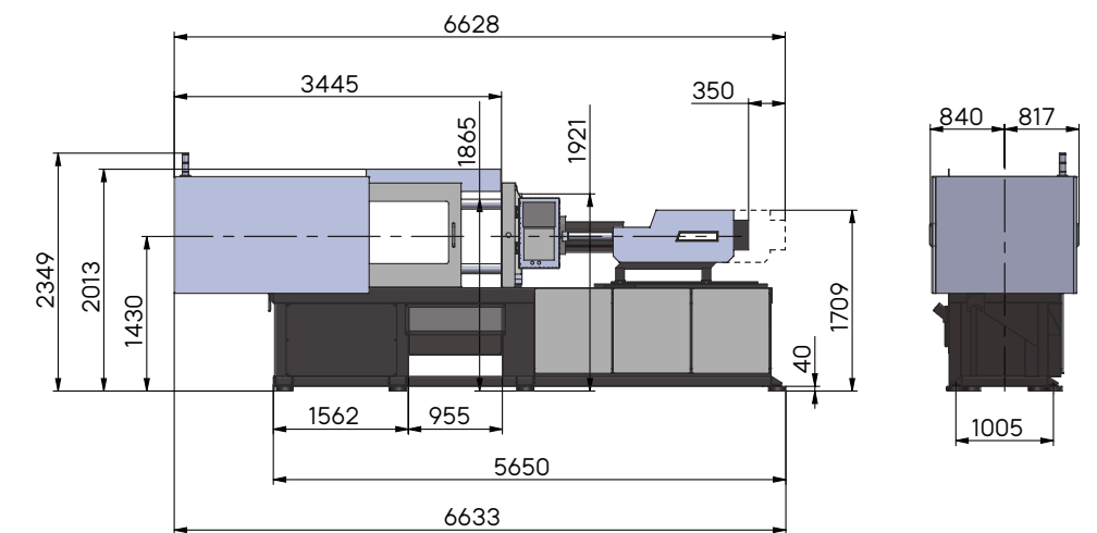
UN320SKIII
