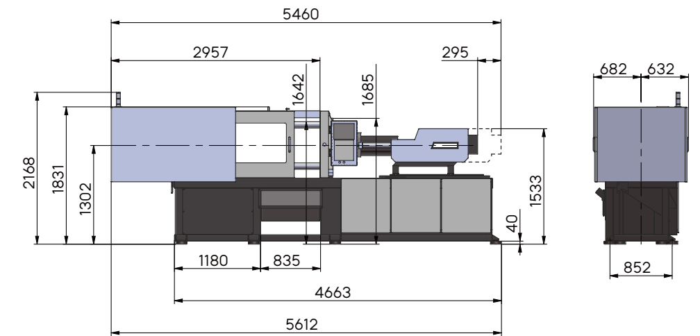
UN200SKIII
