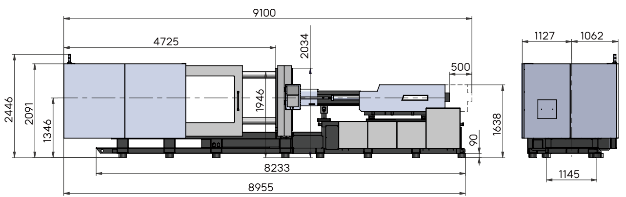
UN650SKIII
