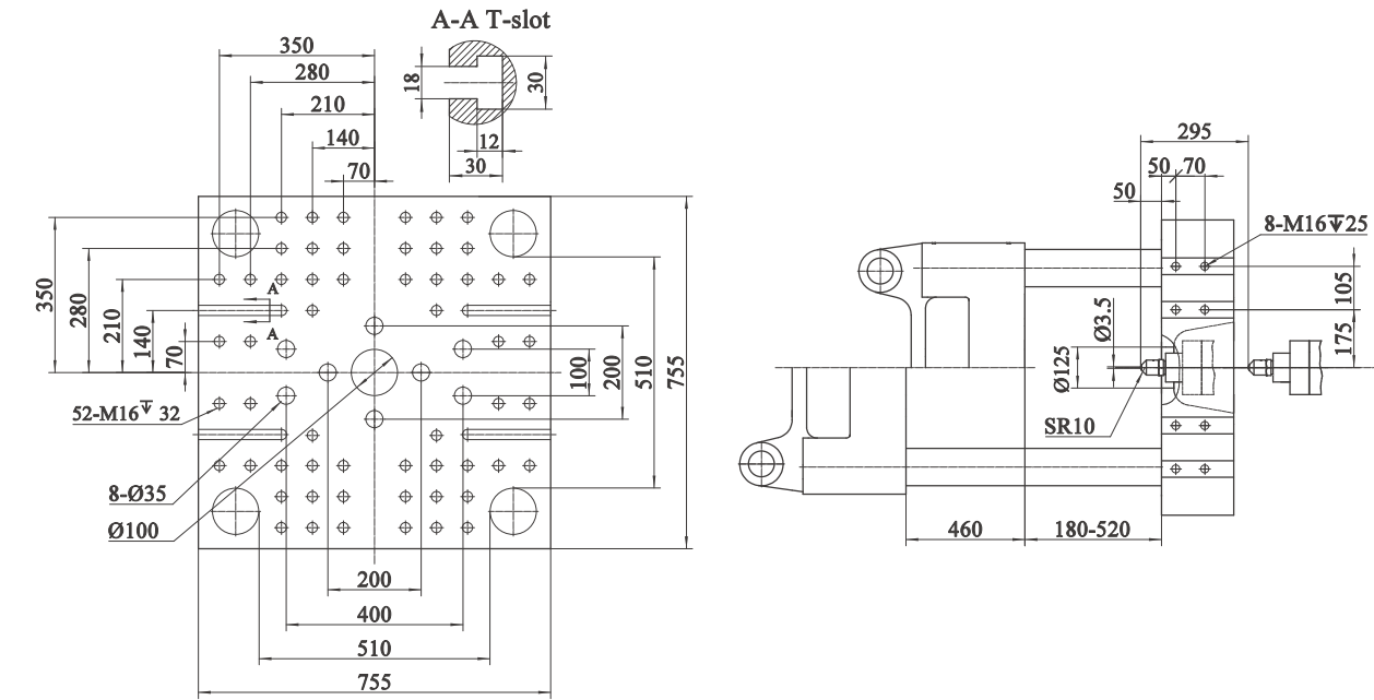
UN200SKIII
