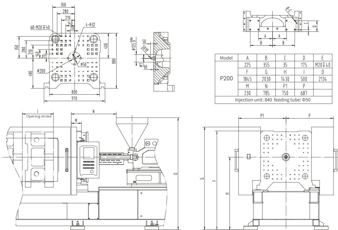
P200 Platen Dimension Drawings
